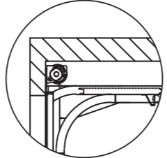
Detail: Front mount spring
