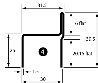
Lock Post
