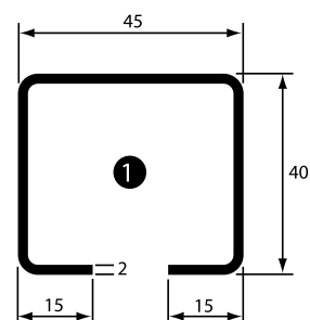
Top Track
