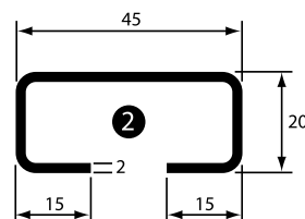
Fixing Frame
