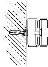
Reveal Fixed Side Frame Detail
